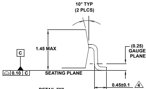
DETAIL "X"
