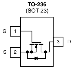
Top View Si2324DS (D4)* * Marking Code
