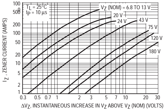
Figure 4. Dynamic Impedance
