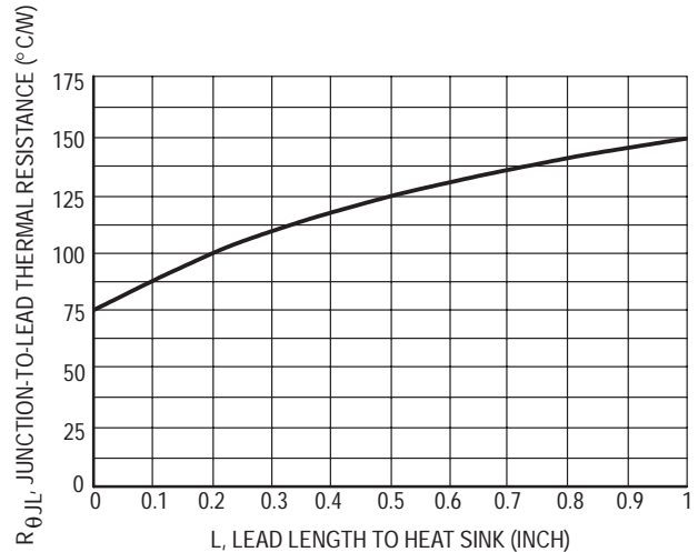
Figure 15. Typical 1N4728 Thermal Resistance versus Lead Length
