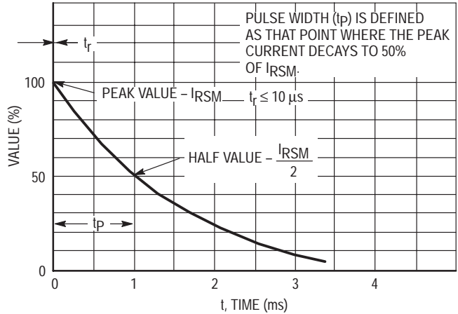
Figure 2. Pulse Waveform
