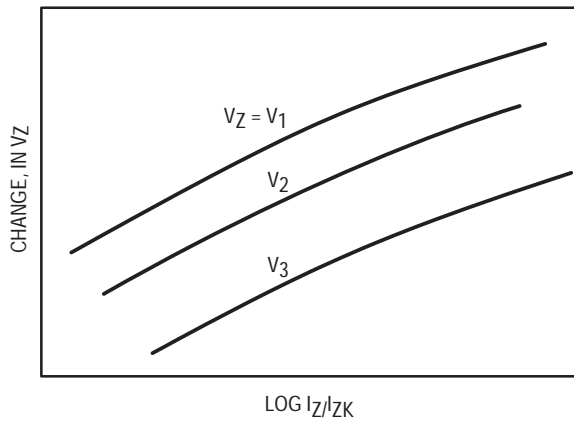
Figure 4. Change in V Z for Changes in I Z
