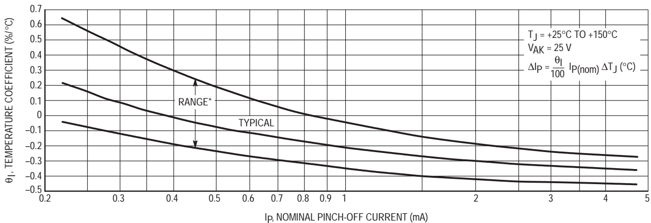
Figure 4. Temperature Coefficient
