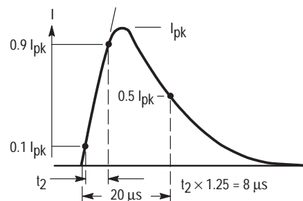
(b) Discharge Current Waveform
