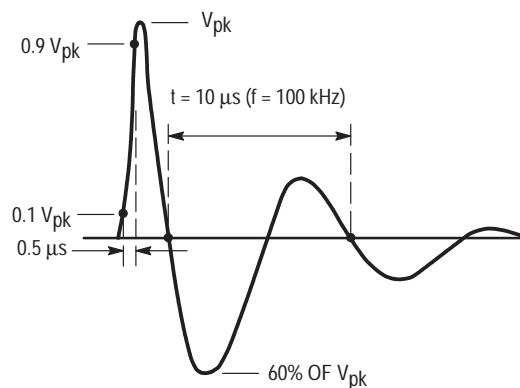
Figure 5. 0.5 \mu s 100 kHz Ring Wave
