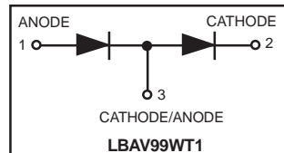
LBAV99RWT1 SOT-323 (SC-70)
