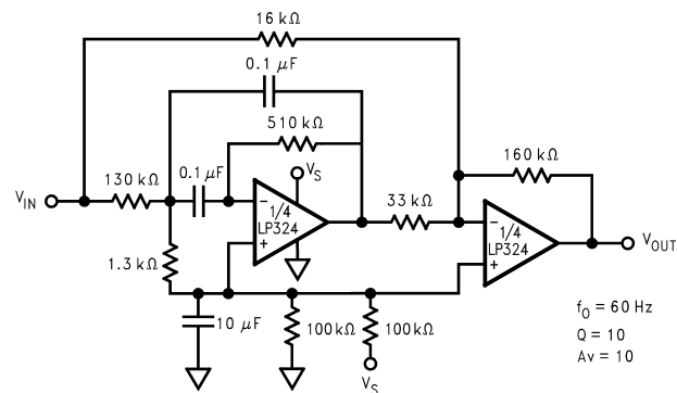
Figure 28. Band-Reject Filter
